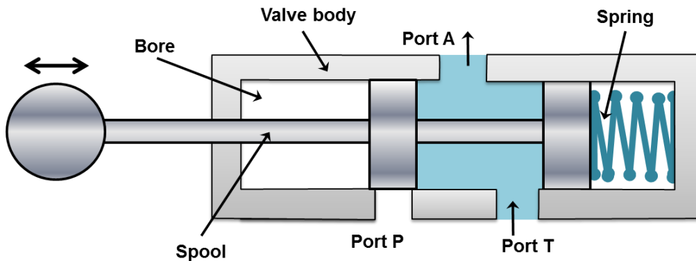
Port A and T connected
