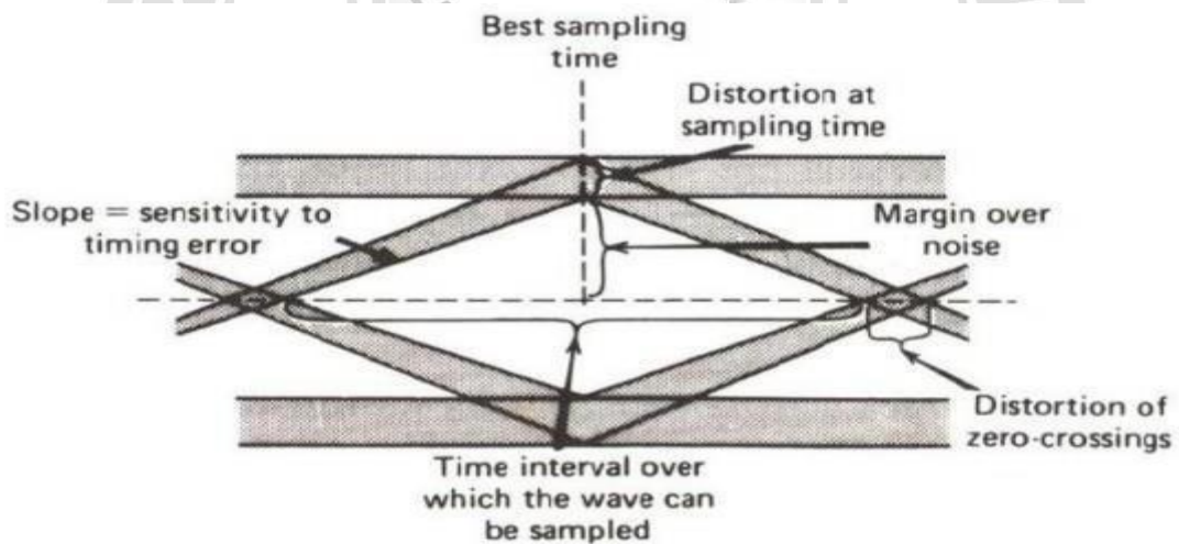
Interpretation of eye pattern
