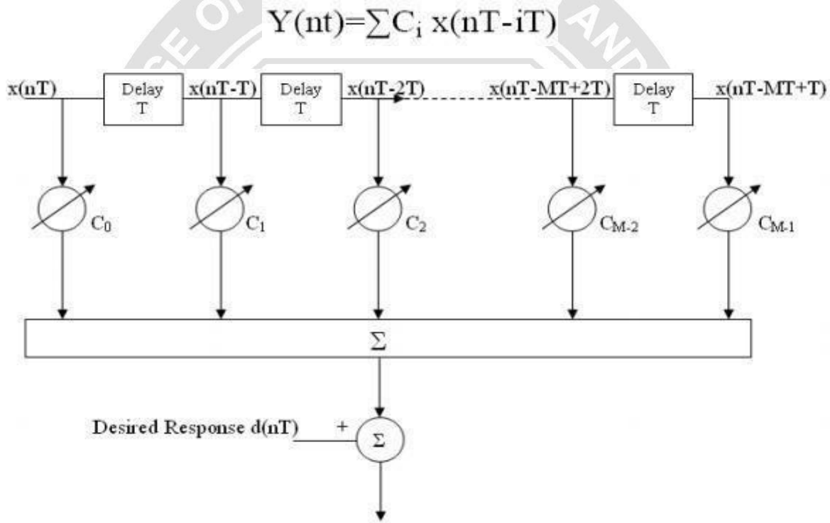
Fig 3.3.1 Adaptive equalization (Source:Brainkart)
