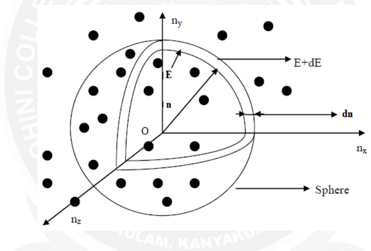
Fig2.5.1-Density of States
