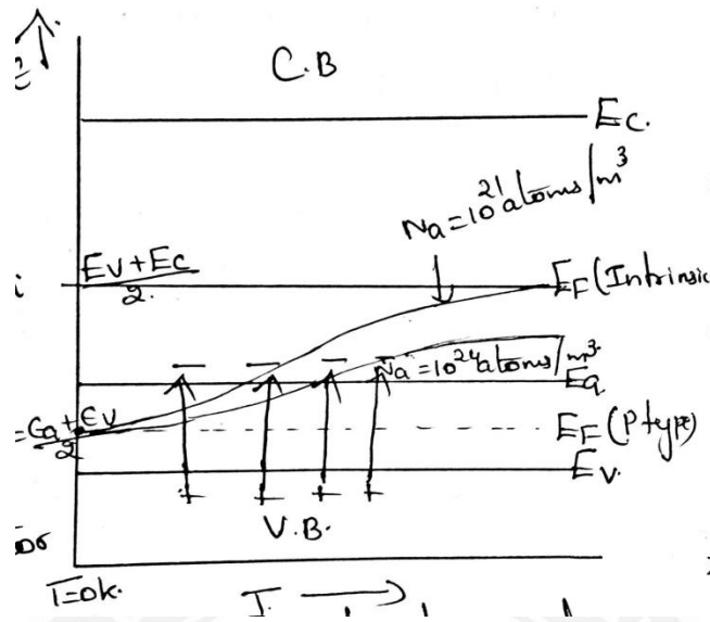
Fig 3.4.2-Variation of Fermi level with temperature for P type semiconductor
