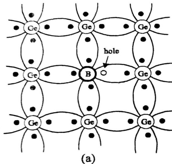
Fig 3.4.1 Crystal structure of P type semiconductor
