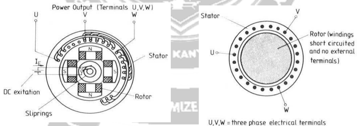
Figure 3.3.3 Wiring of three phase synchronous generator & Induction three-phase asynchronous generator
