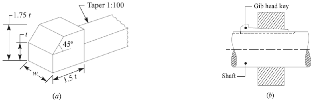
Fig. 2.11. Gib-head key.
