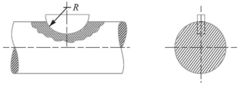
Fig. 2.13. Woodruff key
