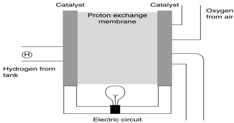
Fig 5.5.6 Proton Exchange Membrane Fuel Cells
