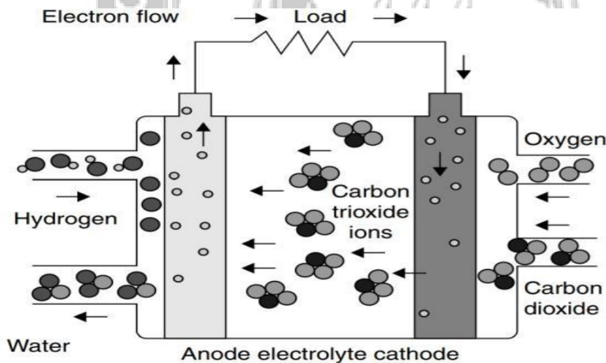
Fig 5.5.4 Molten Carbonate fuel cell
