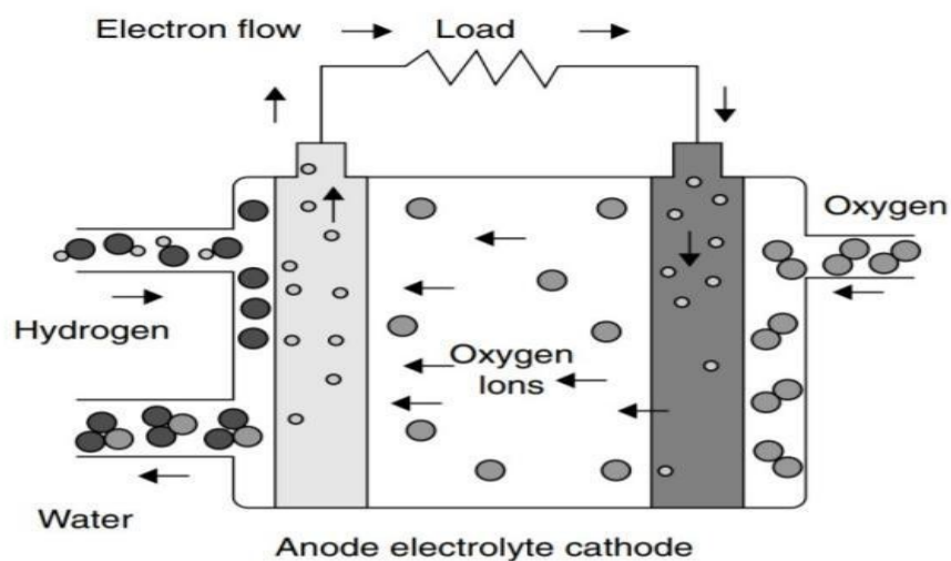
Fig 5.5.6 Solid Oxide Fuel Cell
