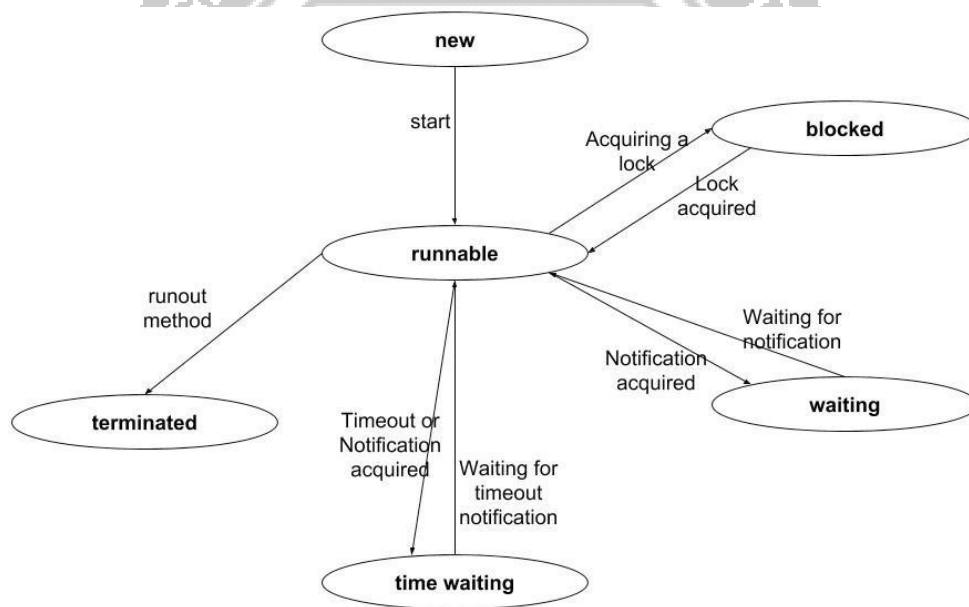
Figure: Life Cycle of a thread
