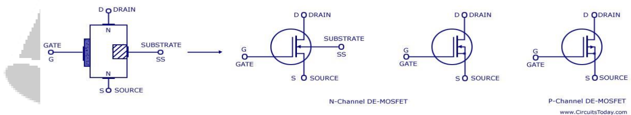
Schematic Symbols For a DE-MOSFET's
