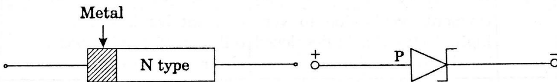
Fig2.8.1 schottky diode and its circuit symbol
