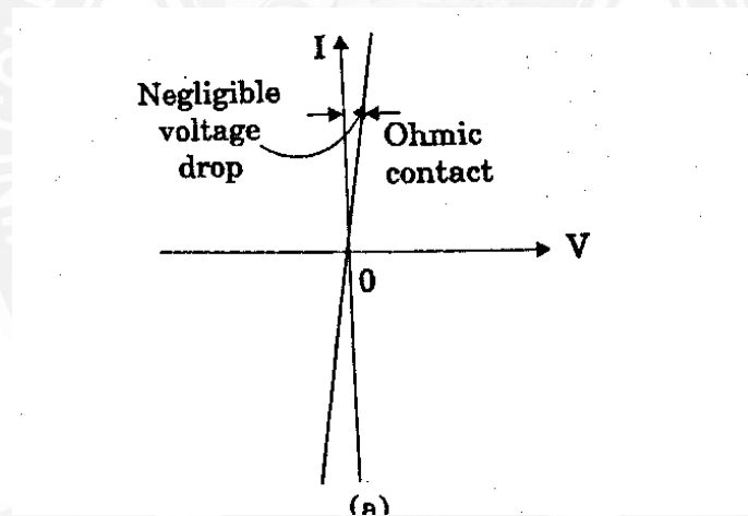
Fig 2.9.3;.V-I Characteristics
