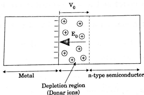
Fig 2.8.2Energy band diagram
