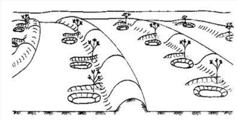
Fig. 28.1. Contour Bunds. (Source: Barron and Salas, 2009)
