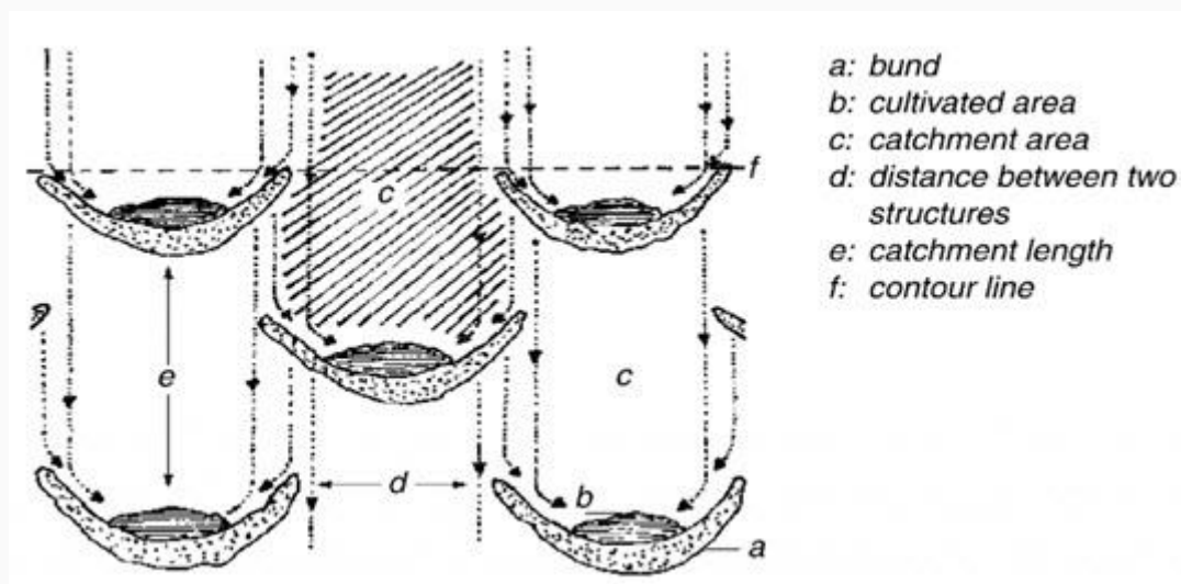
Fig. 28.2. Layout of Semi-Circular Hoop. (Source: Barron and Salas 2009)
