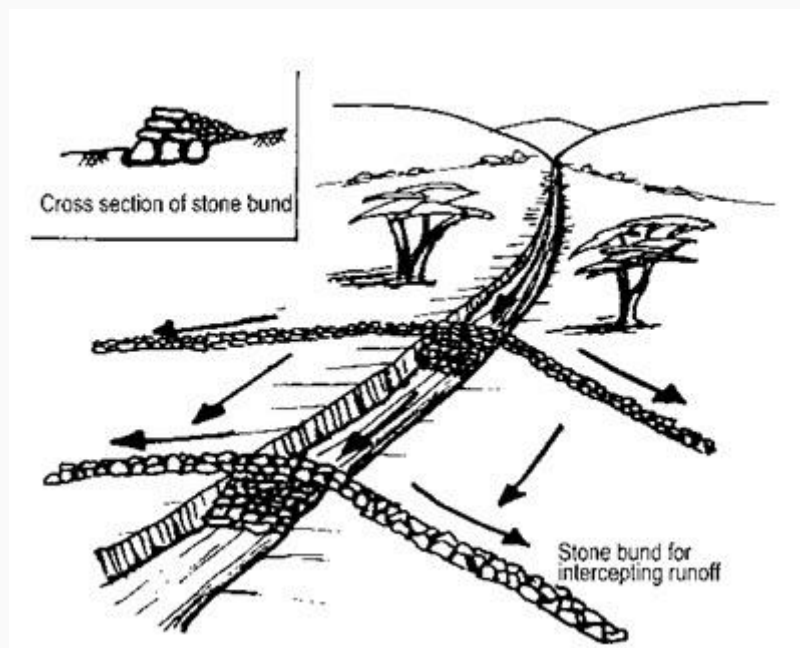
Fig. 28.5. Permeable Rock Dams. (Source: Barron and Salas, 2009)
