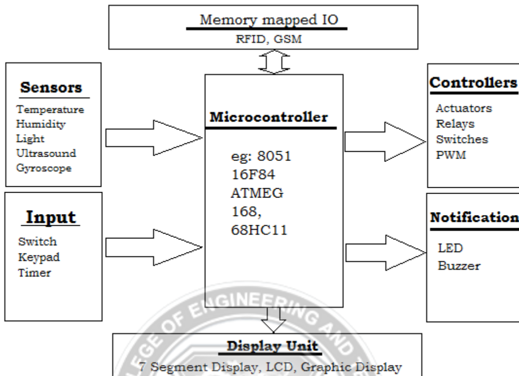
Fig: Basic Embedded System
