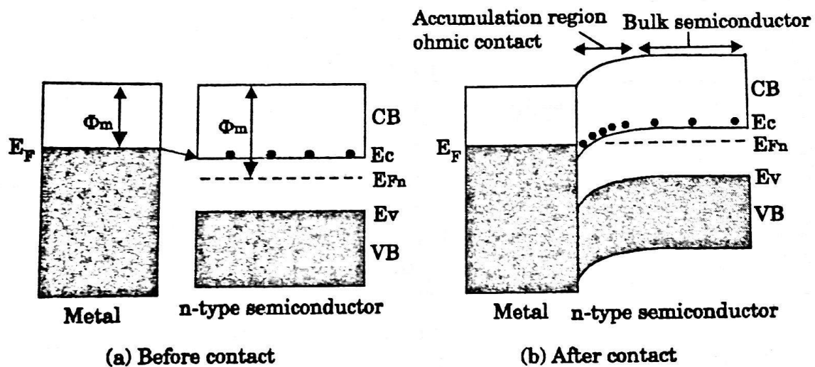
Fig 3.7.1 Ohmic contact before and after contact
