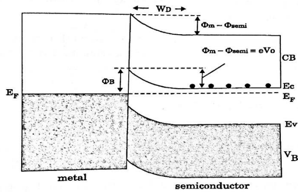
Fig 3.7..3 Formation of depletion layer
