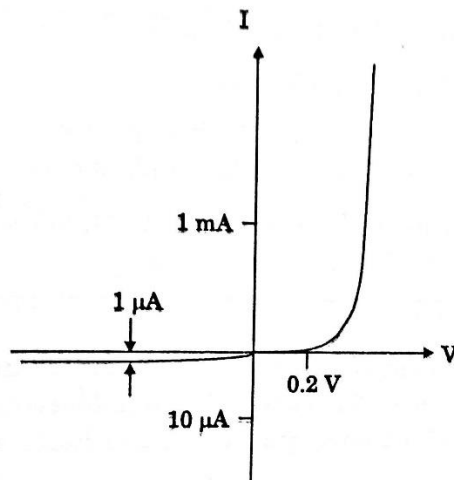
Fig 3.7..4-V-I Characteristics
