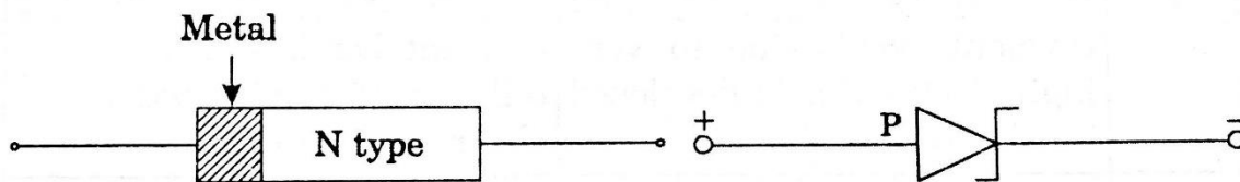
Fig 3.7..1 schottky diode and its circuit symbol
