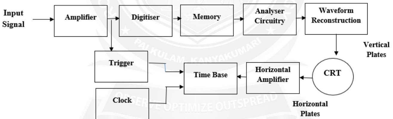
Figure 5.1 Digital Storage Oscilloscope
