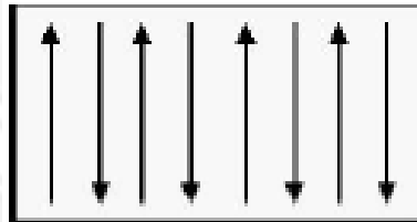
FIG 3.2.1 : Alignment Of Magnetic Moment
