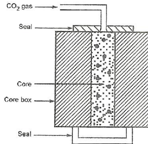
Figure 1.49 CO 2 cores
