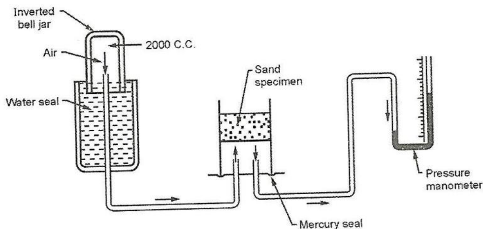
Figure 1.16 Permeability Tester
