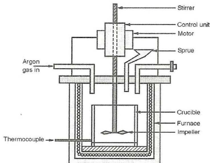
Figure 1.50 Stir Casting
