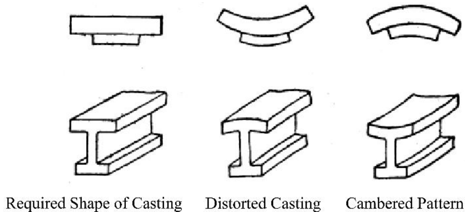
Figure. 1.3. Distortion or Camber Allowance
