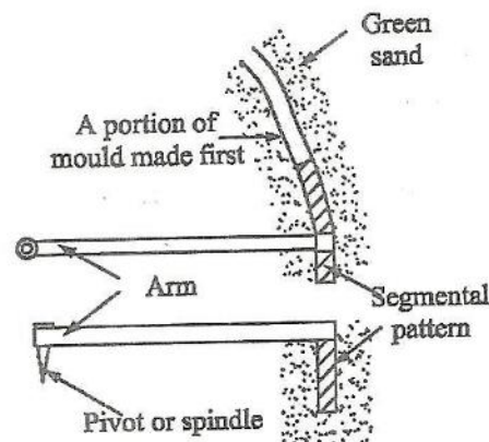
Figure: 1.12 Segmental pattern
