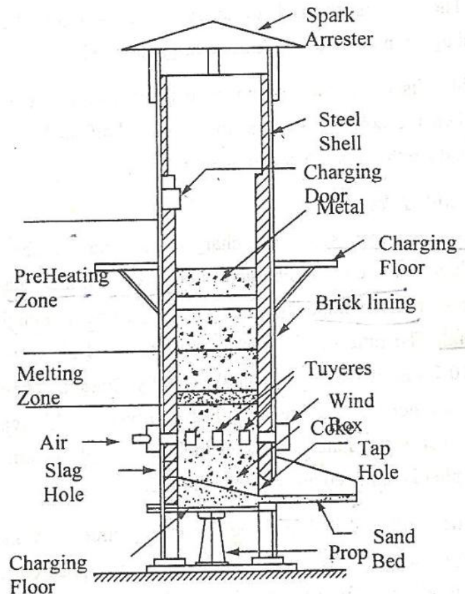
Figure 1.42 Cupola Furnace
