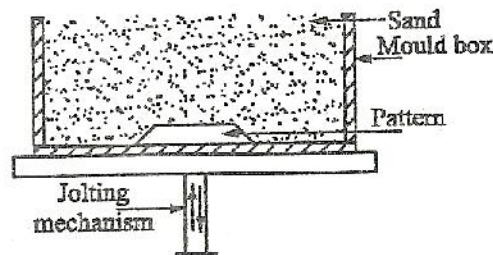
Figure 1.38 Jolt Machine
