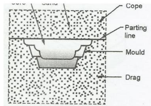
Figure 1.21 Hanging Core
