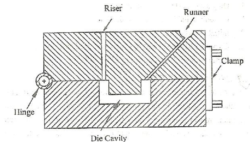
Figure 1.47 Gravity Die Casting
