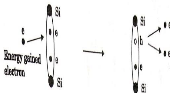
Fig 4.2.3. Impact Ionization
