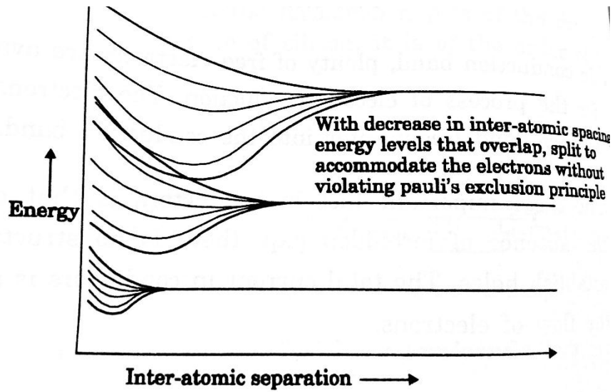
Fig 1.11.1-Tight binding approximation
