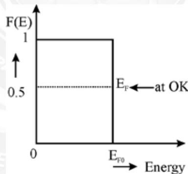
Fig 1.3.1 Fermi level variation with temperature at T=0\text{K}
