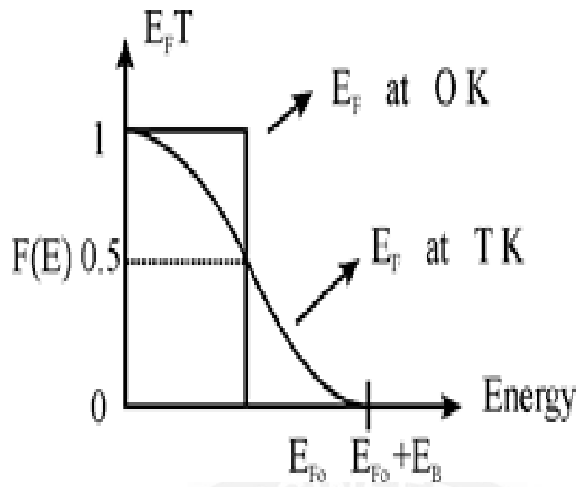
Fig 1.3.2 Fermi level variation with temperature at T
