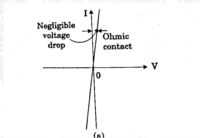
Fig 3.7.3;.V-I Characteristics
