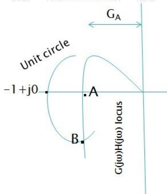
Figure 4.3.1: G(j\omega)H(j\omega) locus
