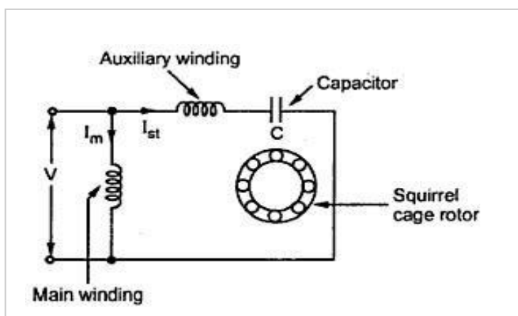
Fig.5.3.4 Capacitor start capacitor run motor
