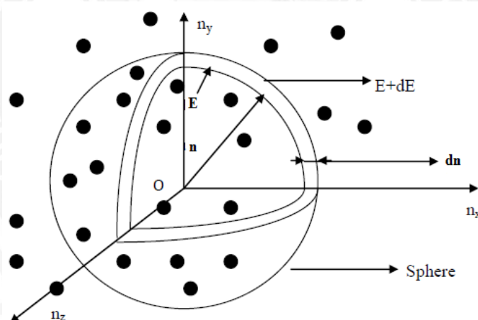
Fig2.5.1-Density of States
