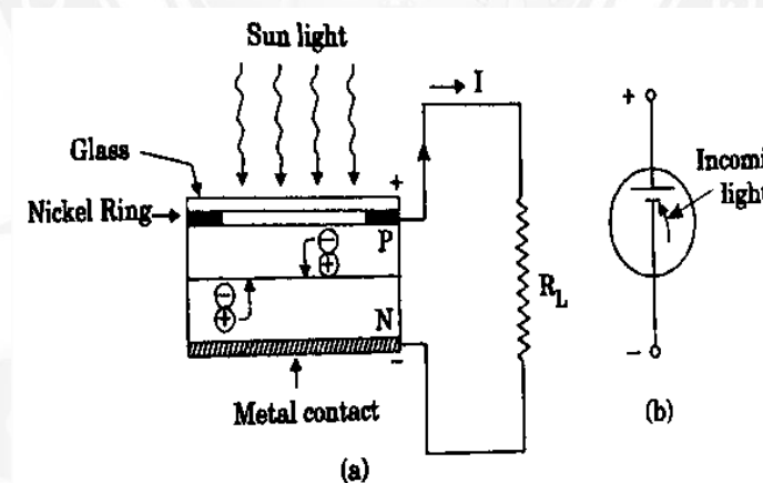
Fig 5.5.1 Solar cell
