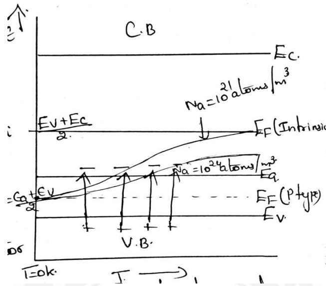
Fig 2.5.2-Variation of Fermi level with temperature for P type semiconductor
