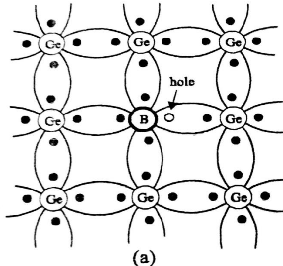
Fig 2.5.1 Crystal structure of P type semiconductor
