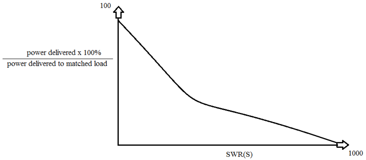
Fig: 2.5.2 Reflection losses as a function of standing wave ratio
