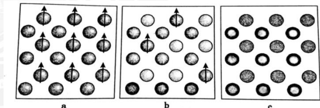
Fig. 5.12 (a) a magnetic semiconductor (e.g. some spinels) (b) a dilute magnetic semiconductor (e.g. (GaMn) As, (InMn), P, ZnCoO etc) (c) a non-magnetic semiconductor (e.g. GaAs, InP, Cu 2 O, NiO etc)
