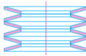
Fig. 1.5 Disc or belleville springs.
