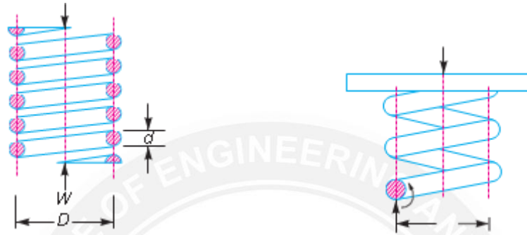
(a) Axially loaded helical spring.
