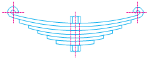
Fig. 1.4 Laminated or leaf springs.
