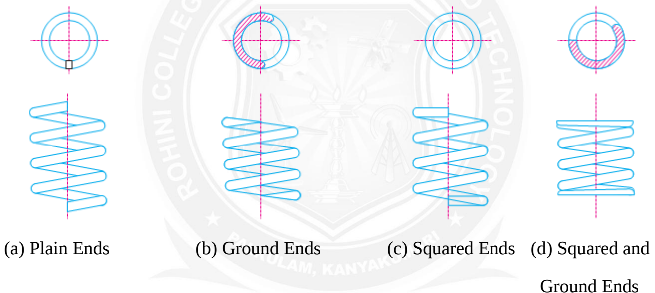
Fig 1.7 End connections for compression helical spring.
