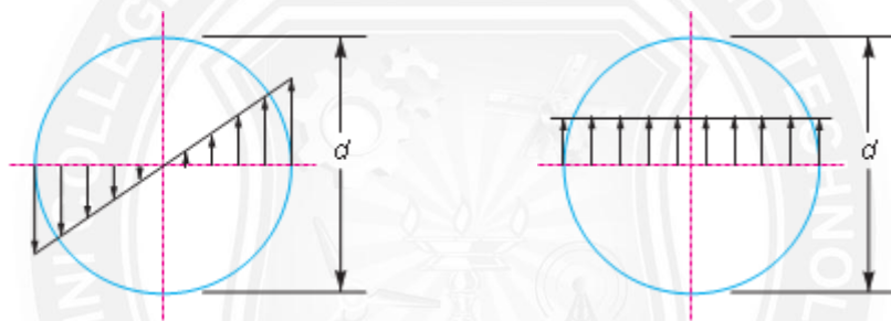
(a) Torsional shear stress diagram. (b) Direct shear stress diagram.
