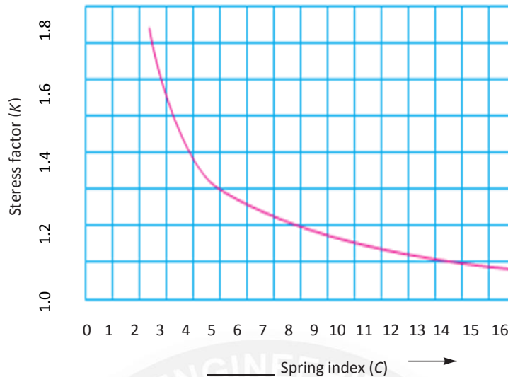
Fig. 1.12. Wahl's stress factor for helical springs.
