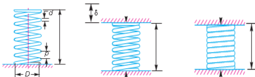
Fig 1.6 Compression spring nomenclature.
