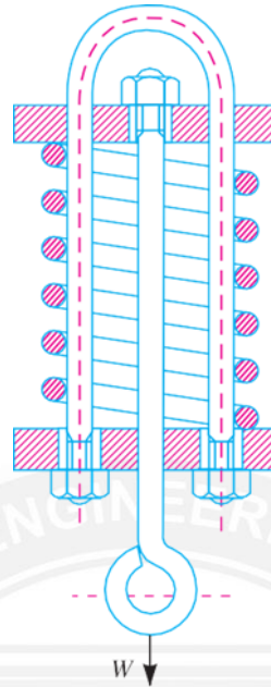
Fig 1.9 Compression spring for carrying tensile load.
