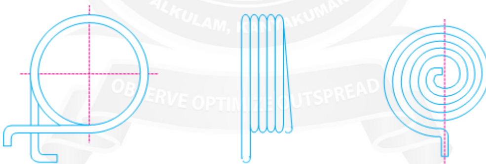
(a) Helical torsion spring.
