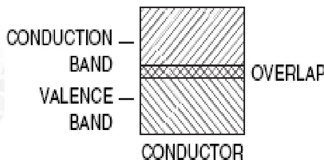
Fig 1.1-Band gap of metal
