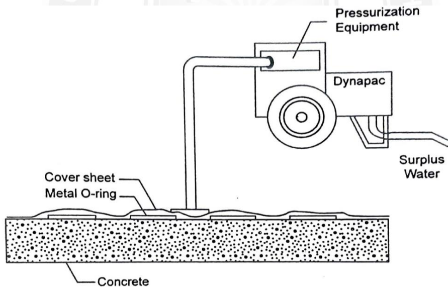
Vacuum concreting
