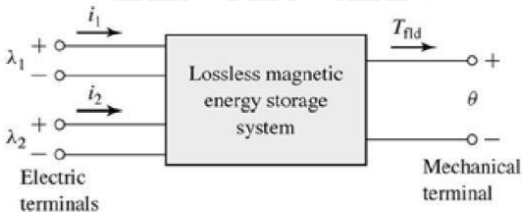
Figure 3.2.2 Electromechanical System
