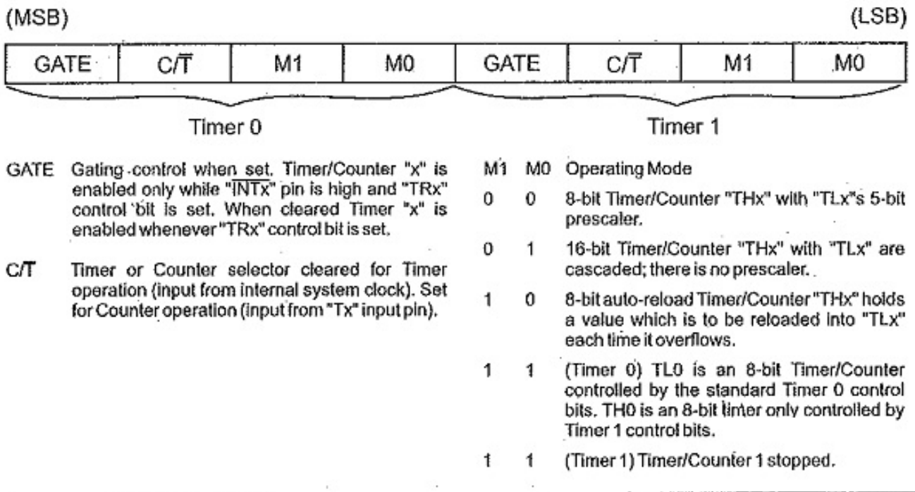
Figure 5.1.2 TMOD Register
