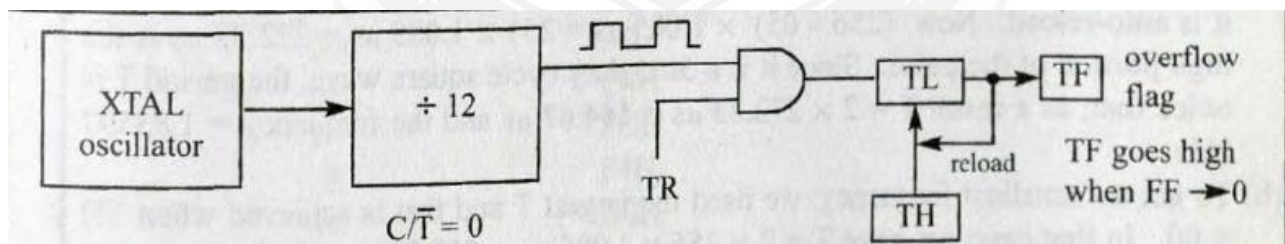
Figure 5.1.4 Timer in Mode 2
