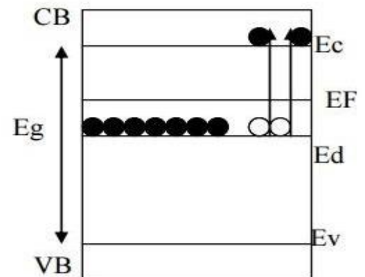
Fig 3.3.2–Energy band diagram for N type semiconductor
