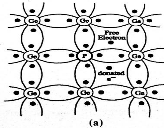
Fig 3.3.1 crystal structure-N type semiconductor
