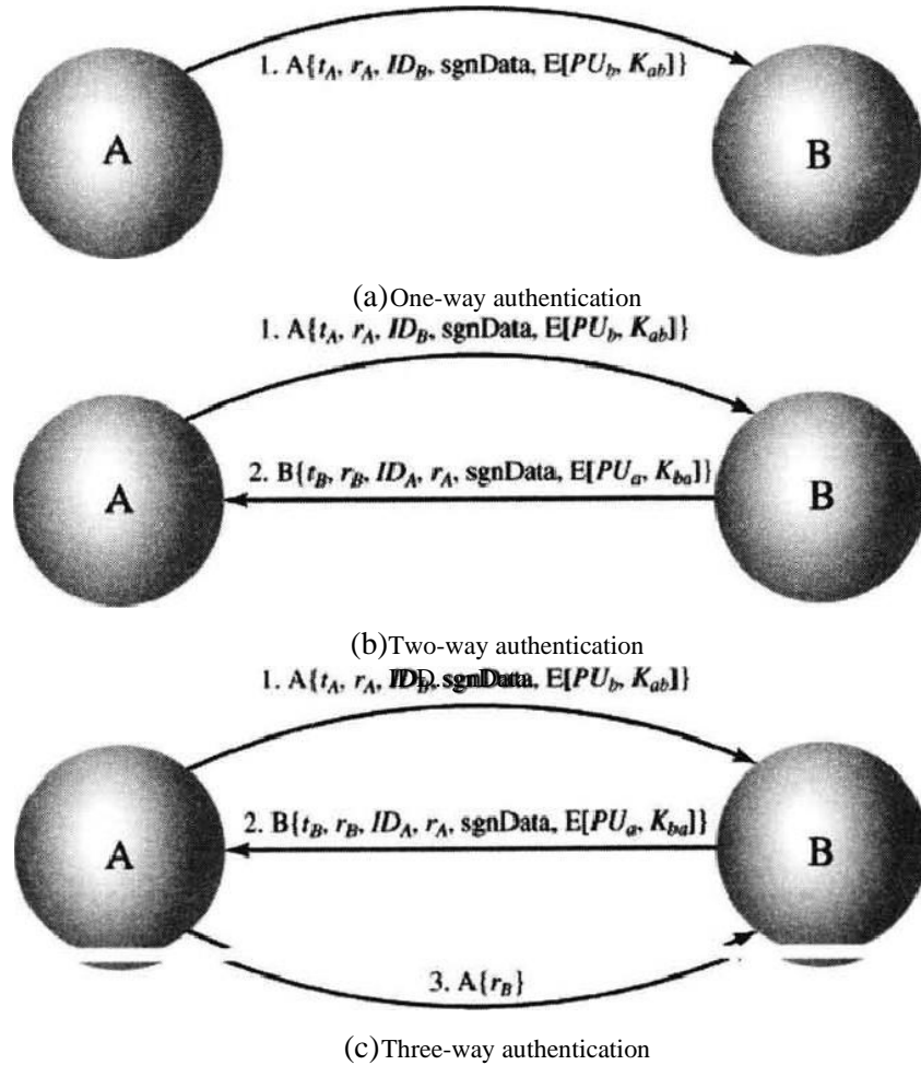
Figure 1.6. X.509 Strong Authentication Procedures
