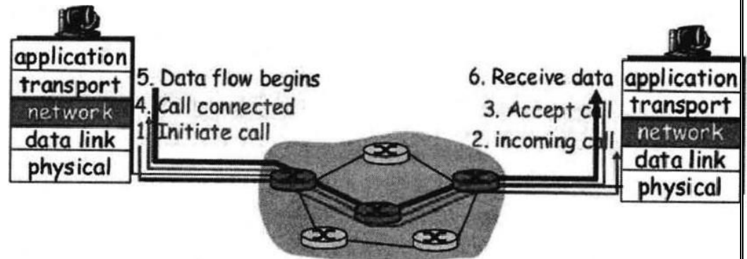
Virtual Circuit
