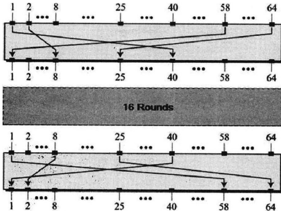
Round Function
